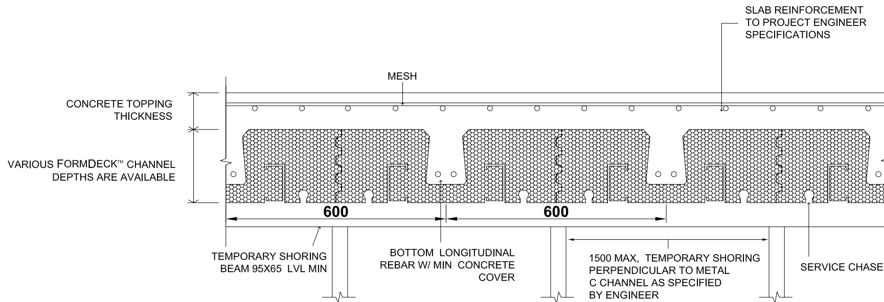
TYPICAL FORMDECK™ SLAB (TRANSVERSE SECTION)
